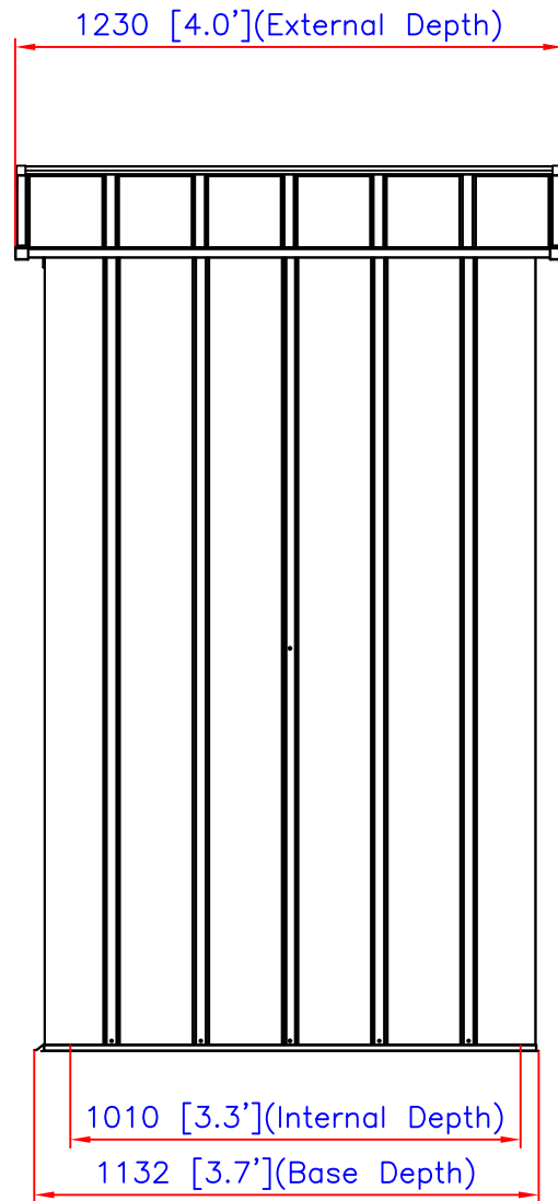
Side View
