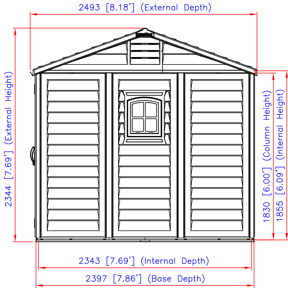
Side View
