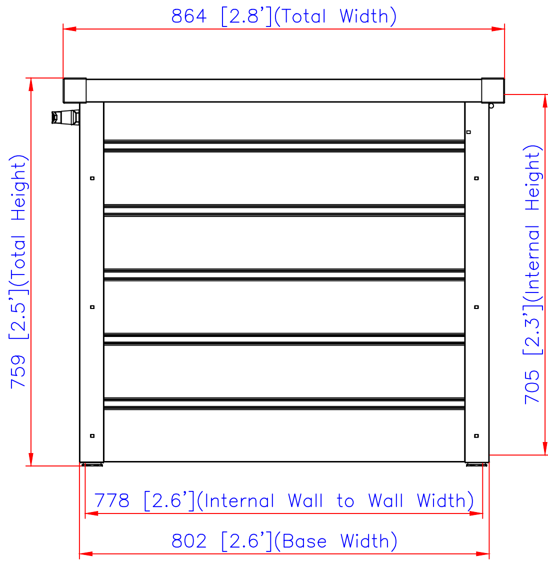
Side View
